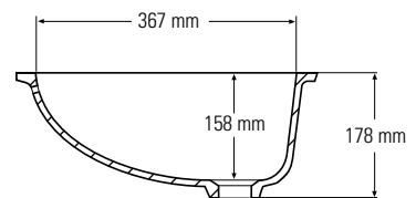
Side cross-section
