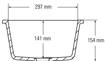
Side cross-section
