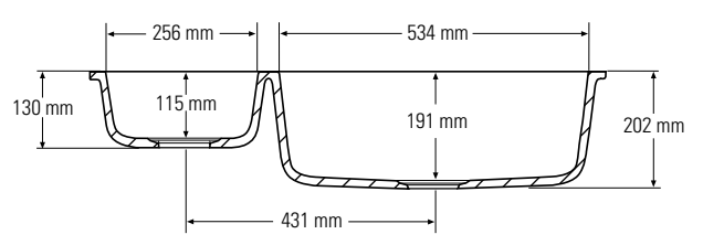
Front cross-section
