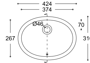
TOP VIEW * overflow
