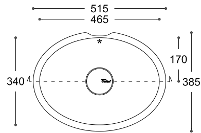
TOP VIEW * overflow
