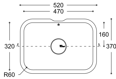
TOP VIEW * overflow
