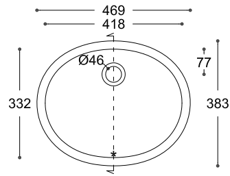
TOP VIEW * overflow
