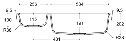
CROSS-SECTION
