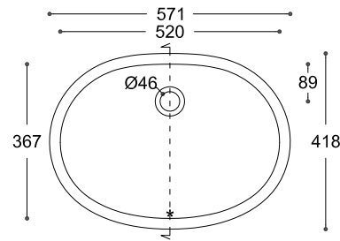
TOP VIEW * overflow
