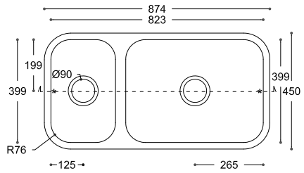
TOP VIEW * overflow
