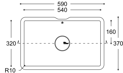
TOP VIEW * overflow
