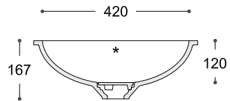
CROSS-SECTION
