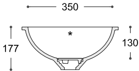
CROSS-SECTION
