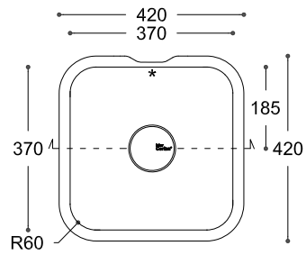
TOP VIEW * overflow
